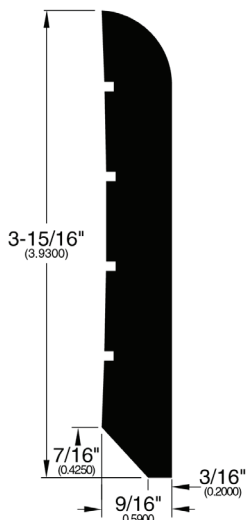
WALL BASE (294)
